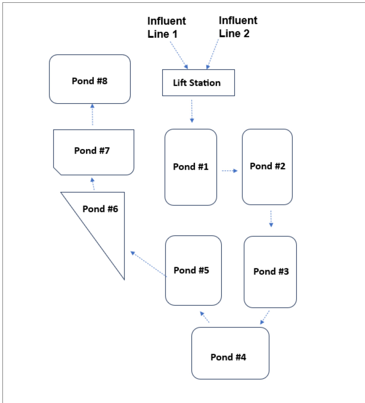
Figure 3. Treatment and Disposal System Process Flow (unlined ponds)
